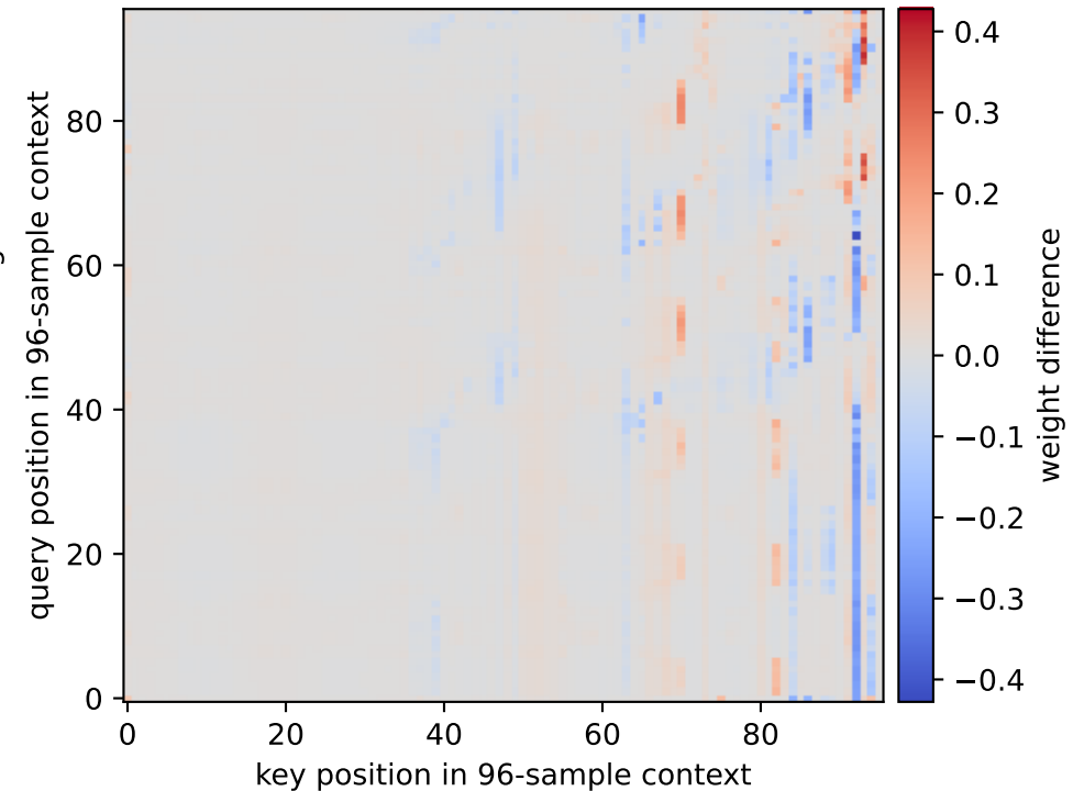
Product A minus Product C: same W_Q, W_K, W_V , different mixing weights
