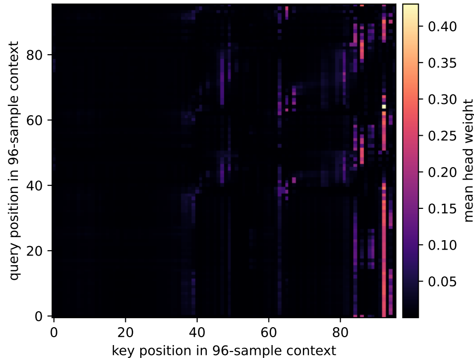
Station 1, Product C: Attention map
