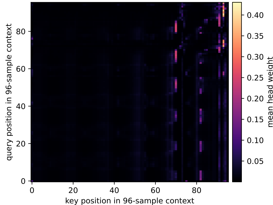
Station 1, Product A: Attention map
